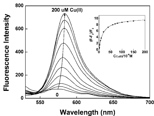
Figure 5. Fluorescence spectra of 1 ( 10\ \mu\text{M} ) in Tris-HCl ( 5\ \text{mM} , \text{pH} = 7.0 ) aqueous buffer solutions in the presence of different amounts of Cu(II). Excitation was performed at 520\ \text{nm} . Inset: fluorescence enhancement factor at 585\ \text{nm} as a function of Cu(II) concentration.
