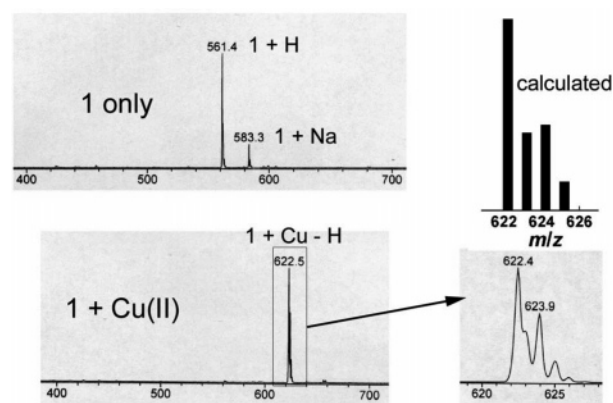
Figure 4. ESI mass spectra (positive) of 1 ( 10\ \mu\text{M} ) in the absence and presence of Cu(II) (1.2 equiv). Right: calculated (top) and observed (bottom) isotopic patterns for the [\text{Cu}(\mathbf{1}-\text{H})]^+ cation, indicating the formation of a 1:1 metal-ligand complex.
