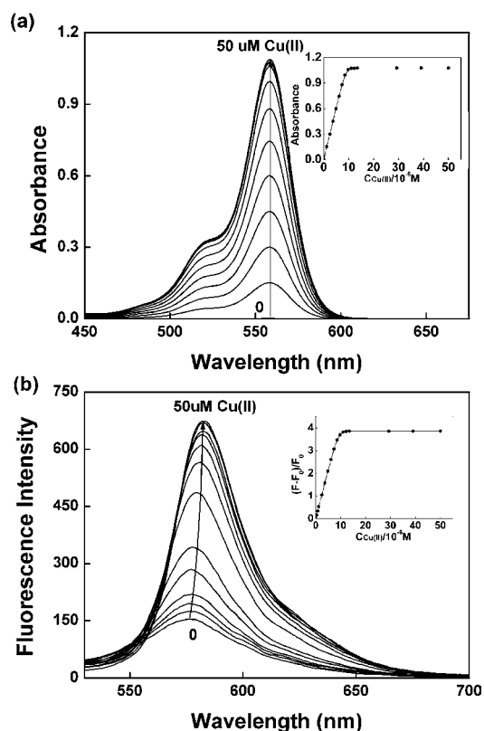
Figure 3. (a) Absorption spectra of 1 ( 10\ \mu\text{M} ) in Tris-HCl ( 10\ \text{mM} , \text{pH} = 7.0 ) buffer containing 50% (v/v) water/ \text{CH}_3\text{CN} in the presence of different amounts of Cu(II). Inset: absorbance at 558 nm as a function of Cu(II) concentration, indicating a 1:1 metal-ligand ratio. (b) Fluorescence spectra of 1 ( 10\ \mu\text{M} ) under the same conditions. Excitation was performed at 520 nm. Inset: fluorescence enhancement factor (F - F_0)/F_0 at 583 nm as a function of Cu(II) concentration.
